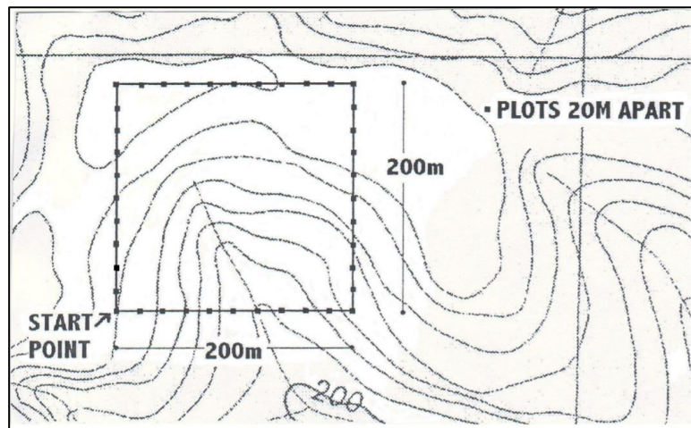
Figure 10: Example of sample point intervals along a square.
